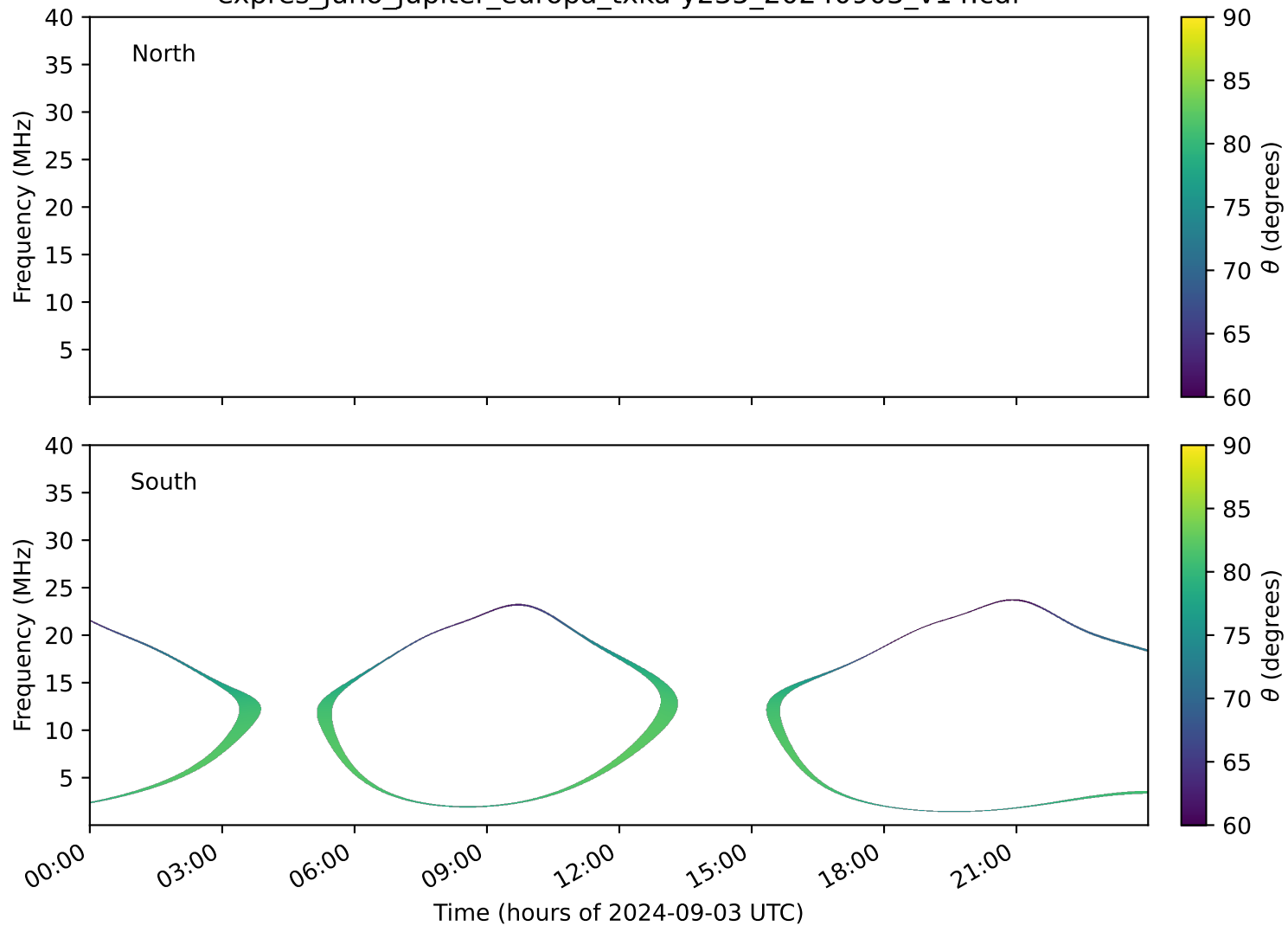
expres_juno_jupiter_europa_txka-y235_20240903_v14.cdf
