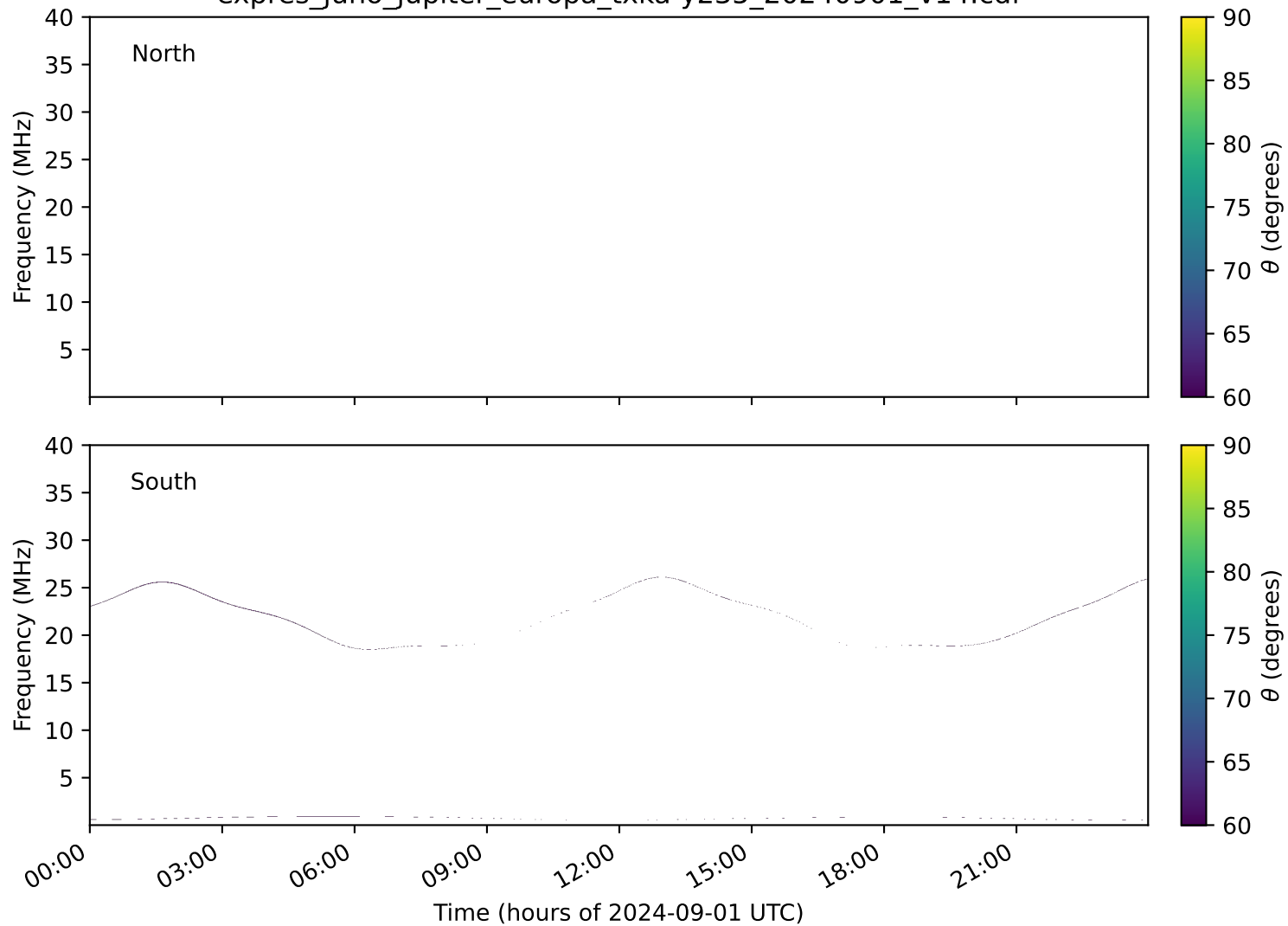
expres_juno_jupiter_europa_txka-y235_20240901_v14.cdf
