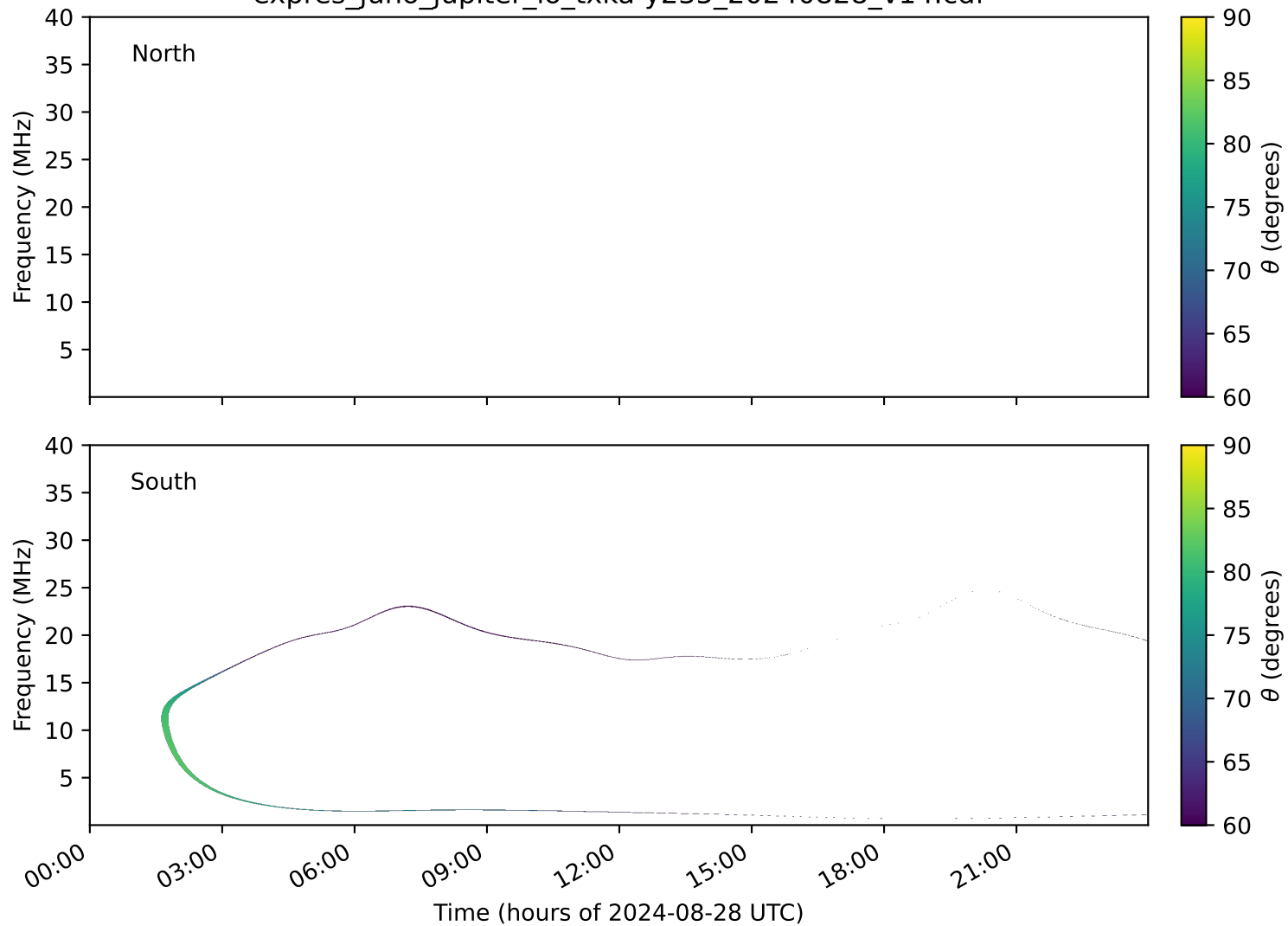
expres_juno_jupiter_io_txka-y235_20240828_v14.cdf
