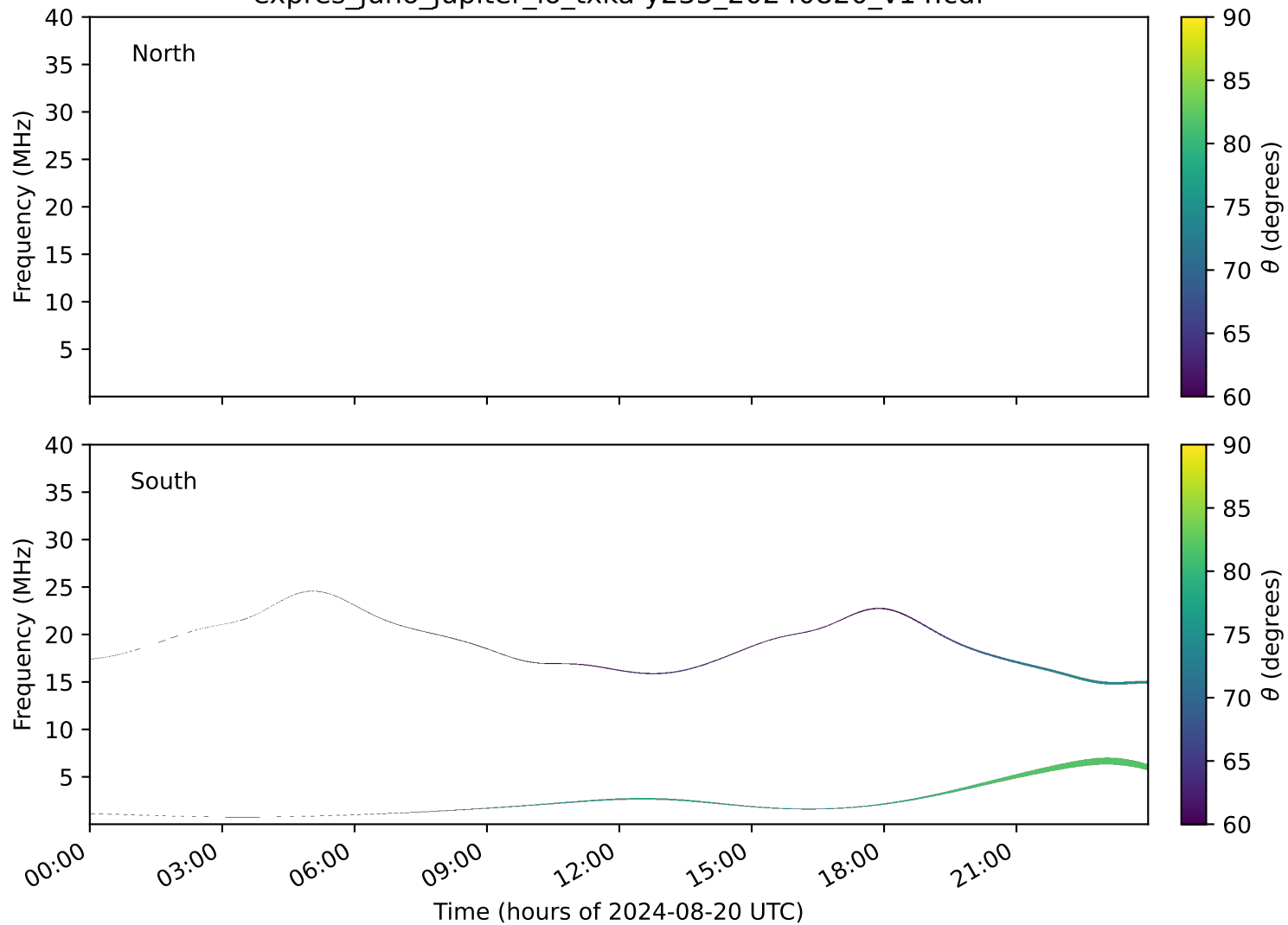
expres_juno_jupiter_io_txka-y235_20240820_v14.cdf
