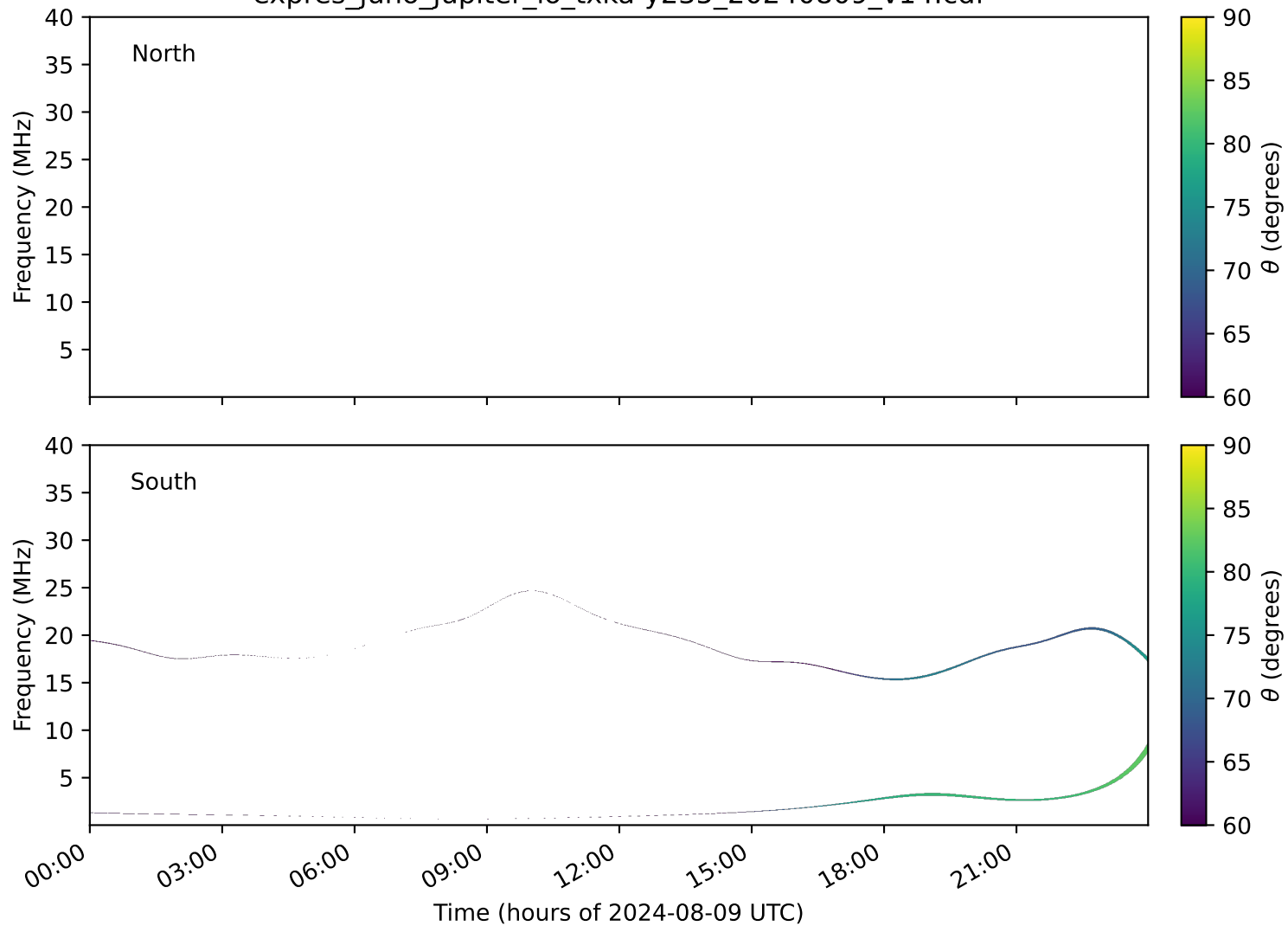
expres_juno_jupiter_io_txka-y235_20240809_v14.cdf
