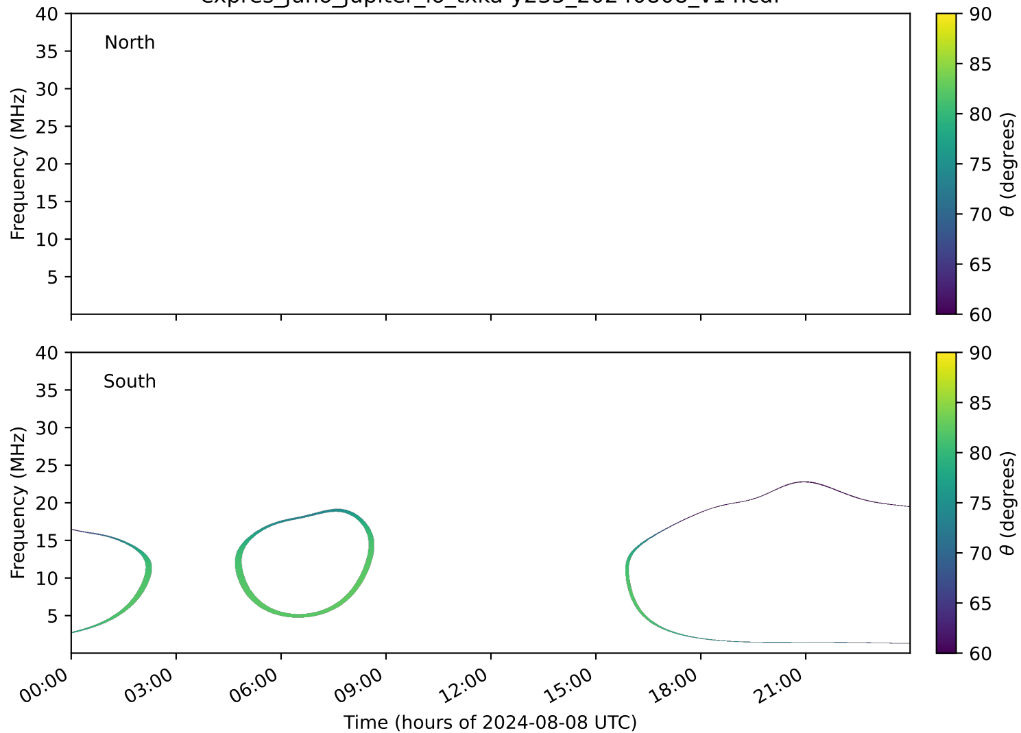
expres_juno_jupiter_io_txka-y235_20240808_v14.cdf
