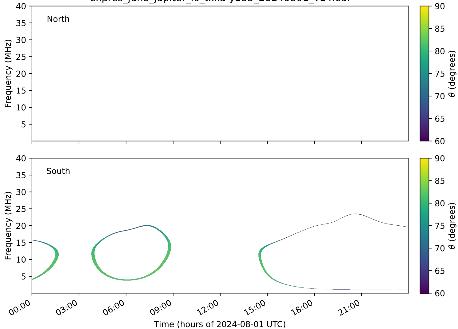
expres_juno_jupiter_io_txka-y235_20240801_v14.cdf
