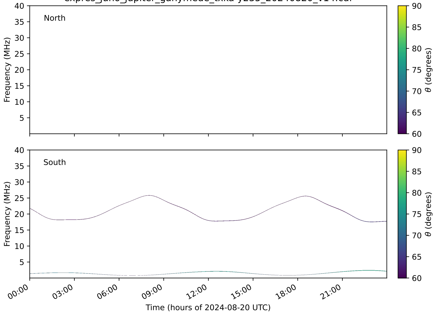
expres_juno_jupiter_ganymede_txka-y235_20240820_v14.cdf
