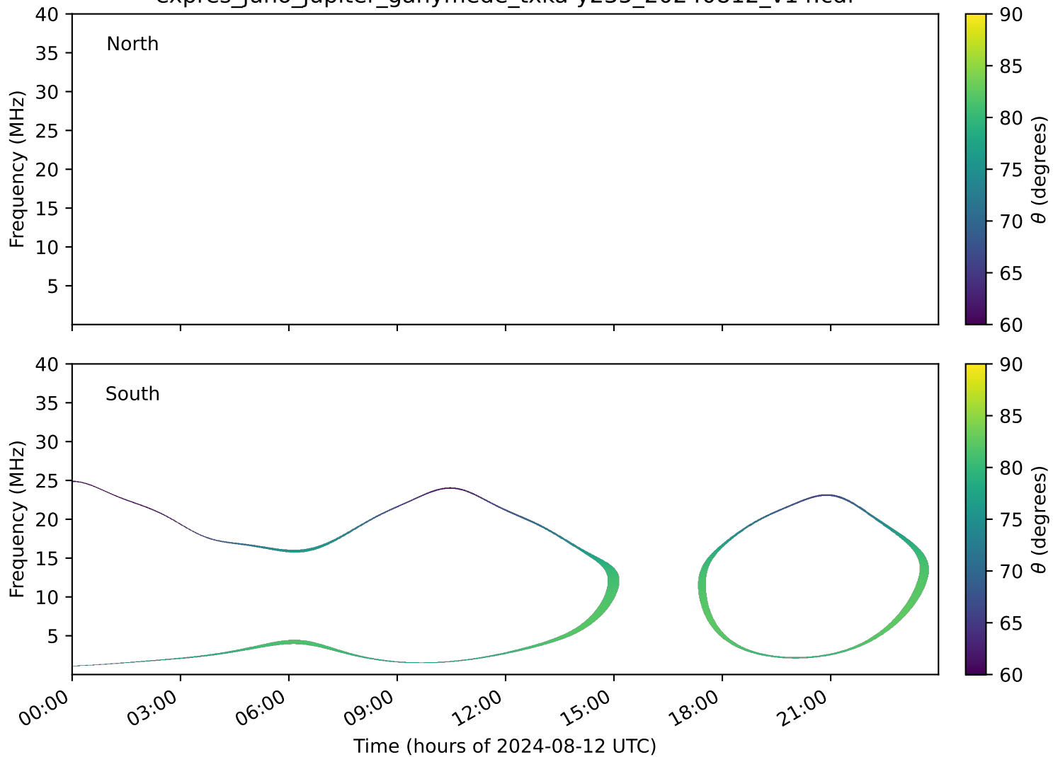
expres_juno_jupiter_ganymede_txka-y235_20240812_v14.cdf
