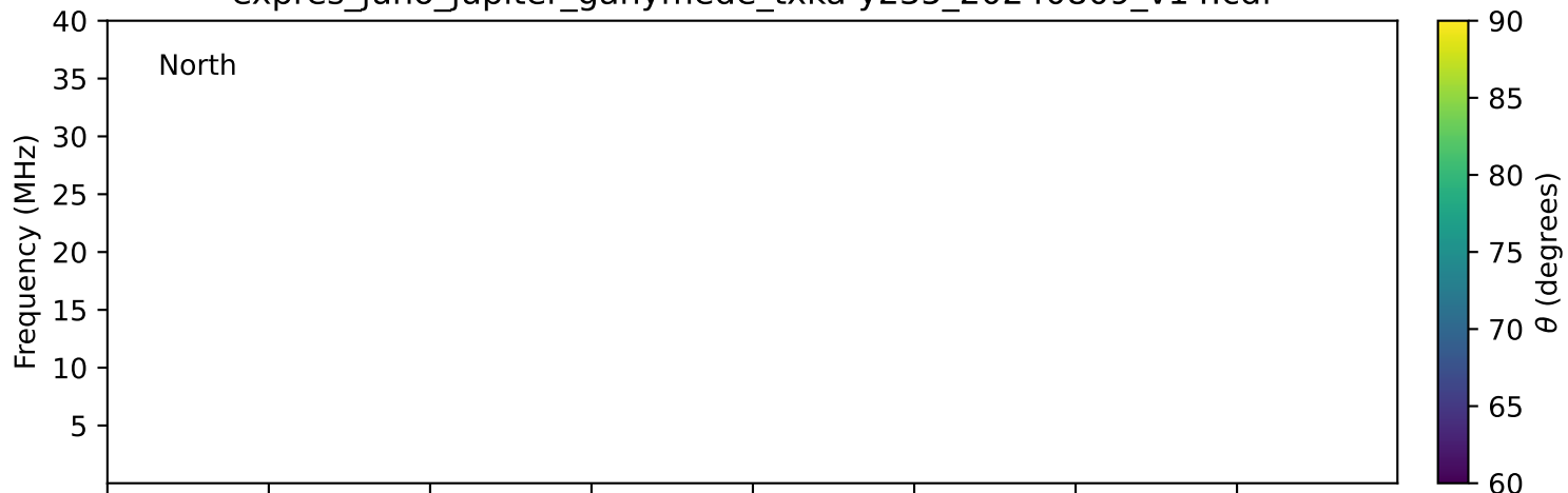
expres_juno_jupiter_ganymede_txka-y235_20240809_v14.cdf
