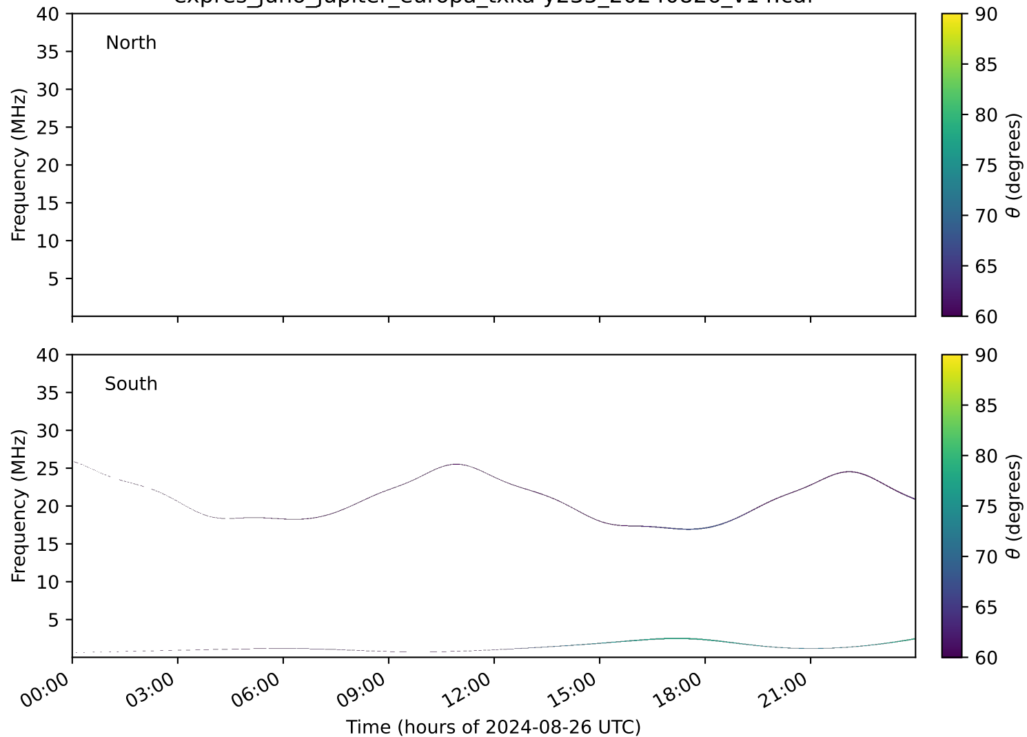
expres_juno_jupiter_europa_txka-y235_20240826_v14.cdf
