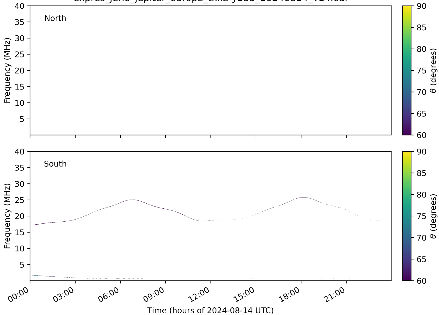
expres_juno_jupiter_europa_txka-y235_20240814_v14.cdf
