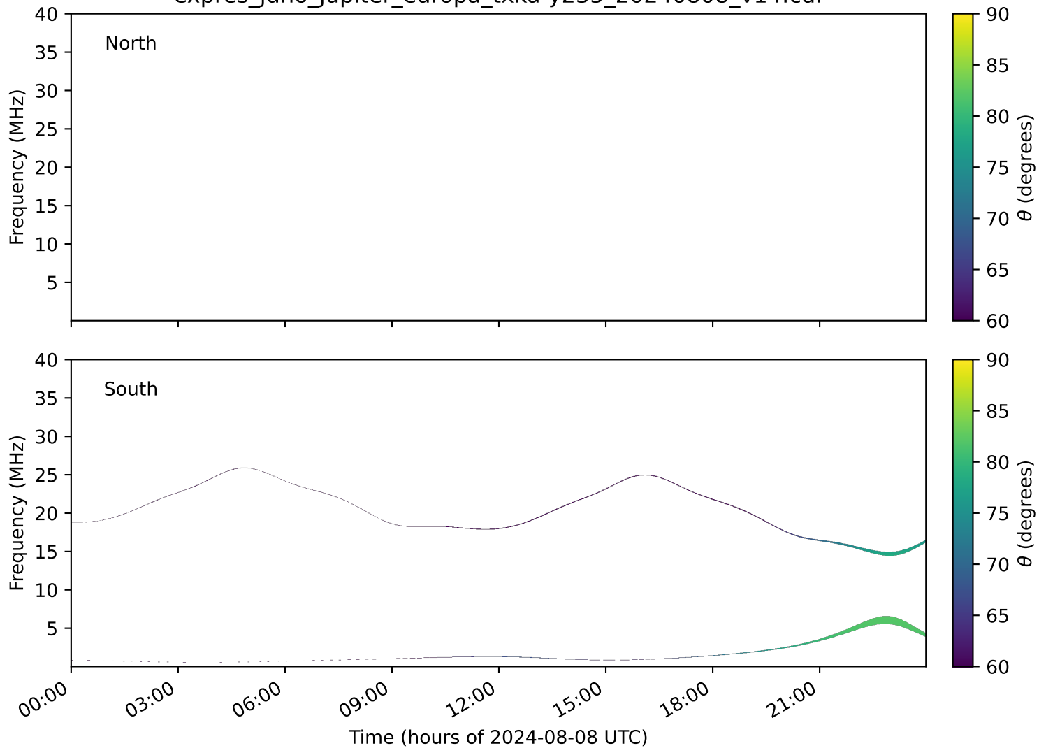
expres_juno_jupiter_europa_txka-y235_20240808_v14.cdf
