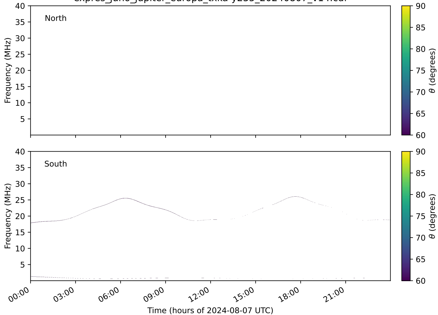
expres_juno_jupiter_europa_txka-y235_20240807_v14.cdf
