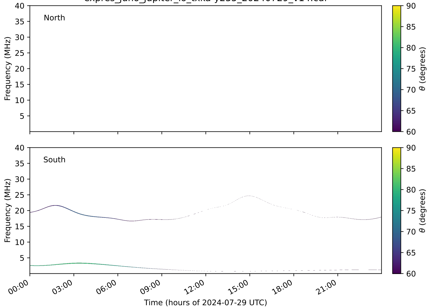
expres_juno_jupiter_io_txka-y235_20240729_v14.cdf
