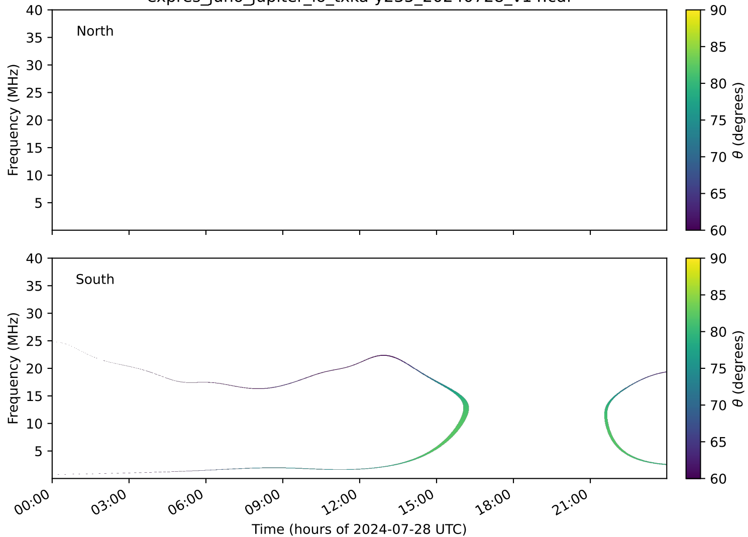
expres_juno_jupiter_io_txka-y235_20240728_v14.cdf
