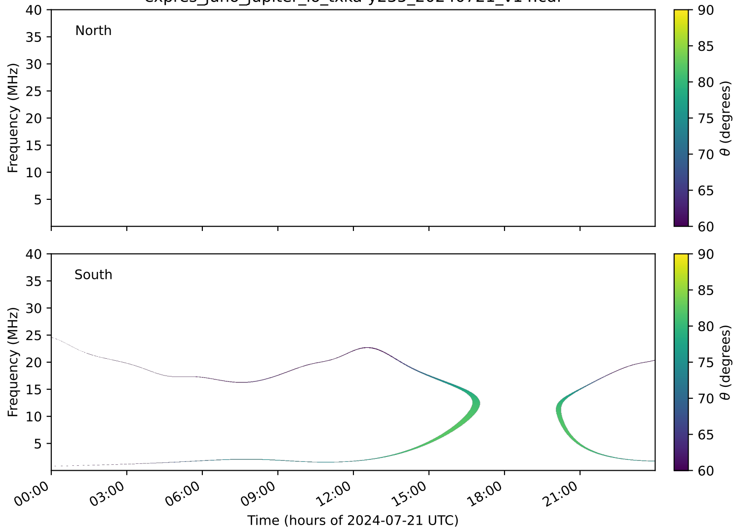
expres_juno_jupiter_io_txka-y235_20240721_v14.cdf
