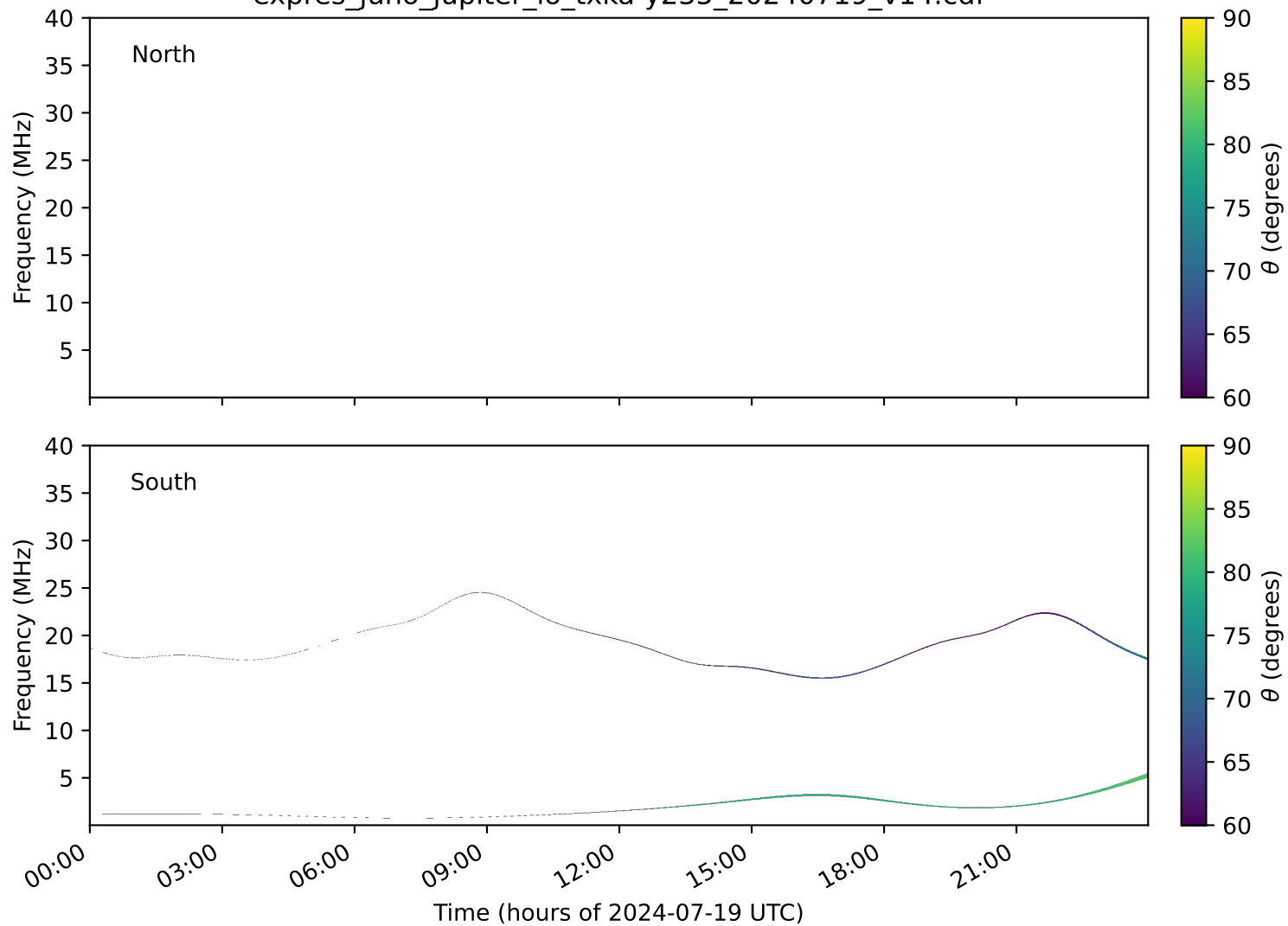
expres_juno_jupiter_io_txka-y235_20240719_v14.cdf
