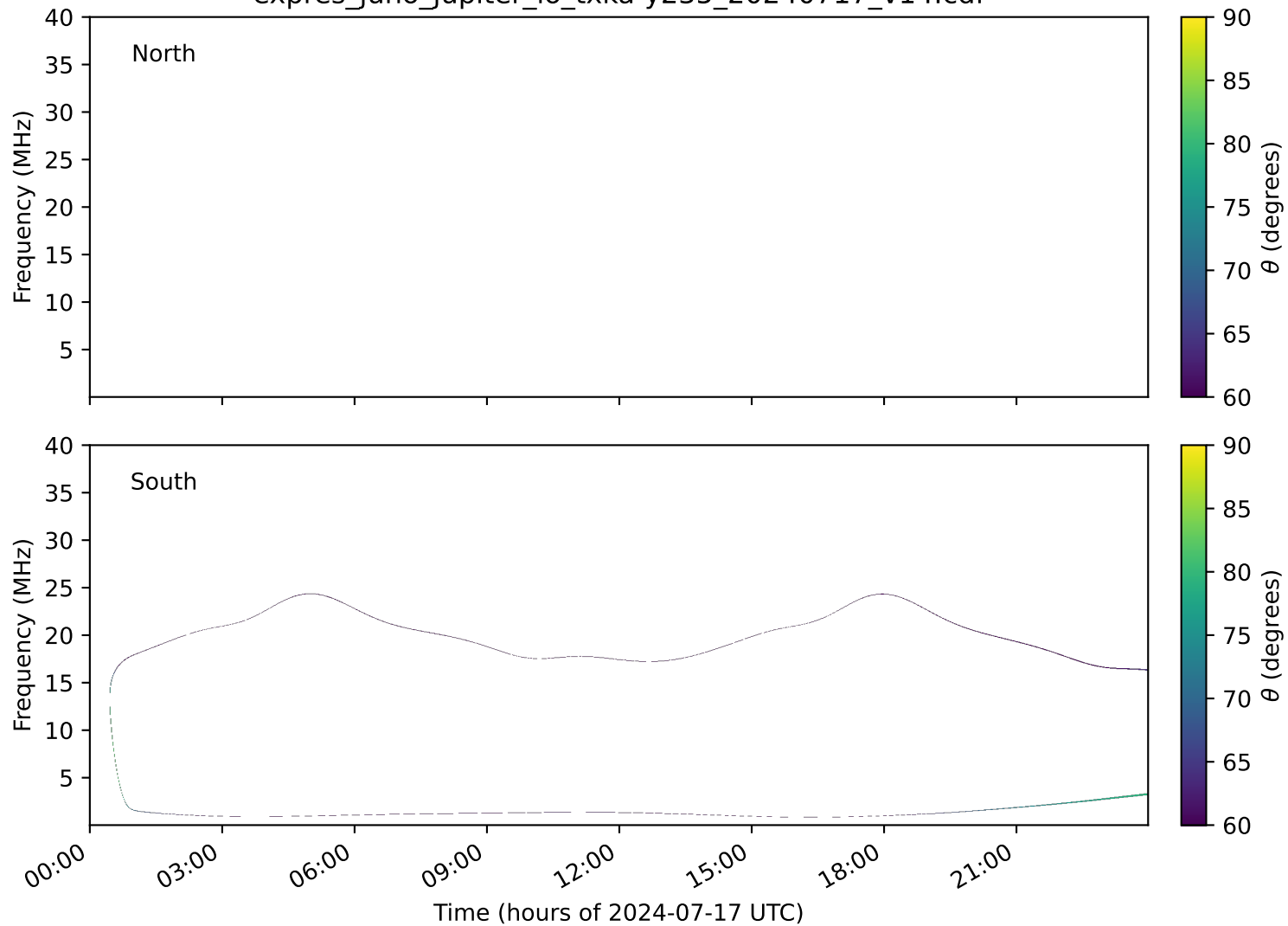
expres_juno_jupiter_io_txka-y235_20240717_v14.cdf
