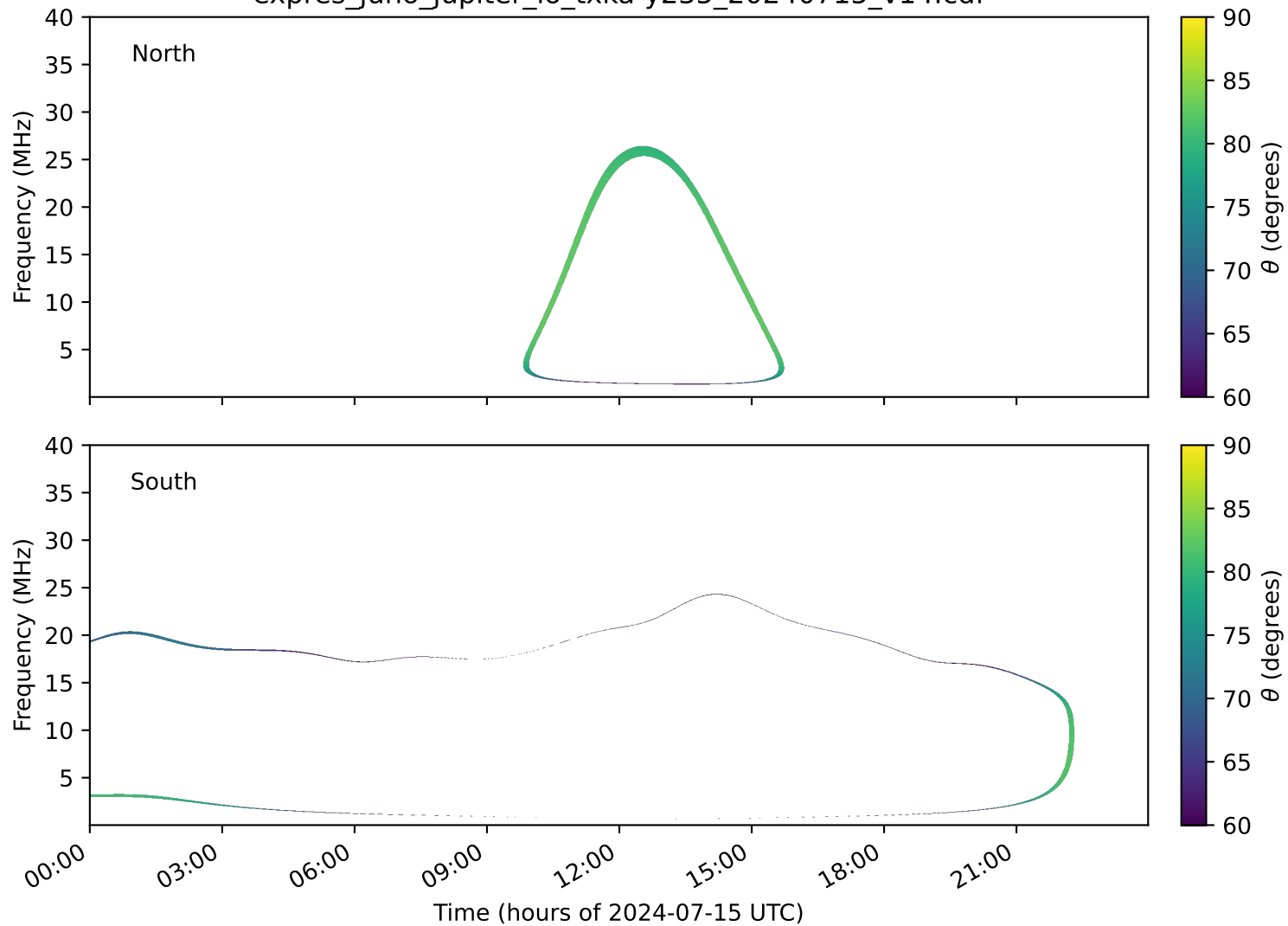
expres_juno_jupiter_io_txka-y235_20240715_v14.cdf
