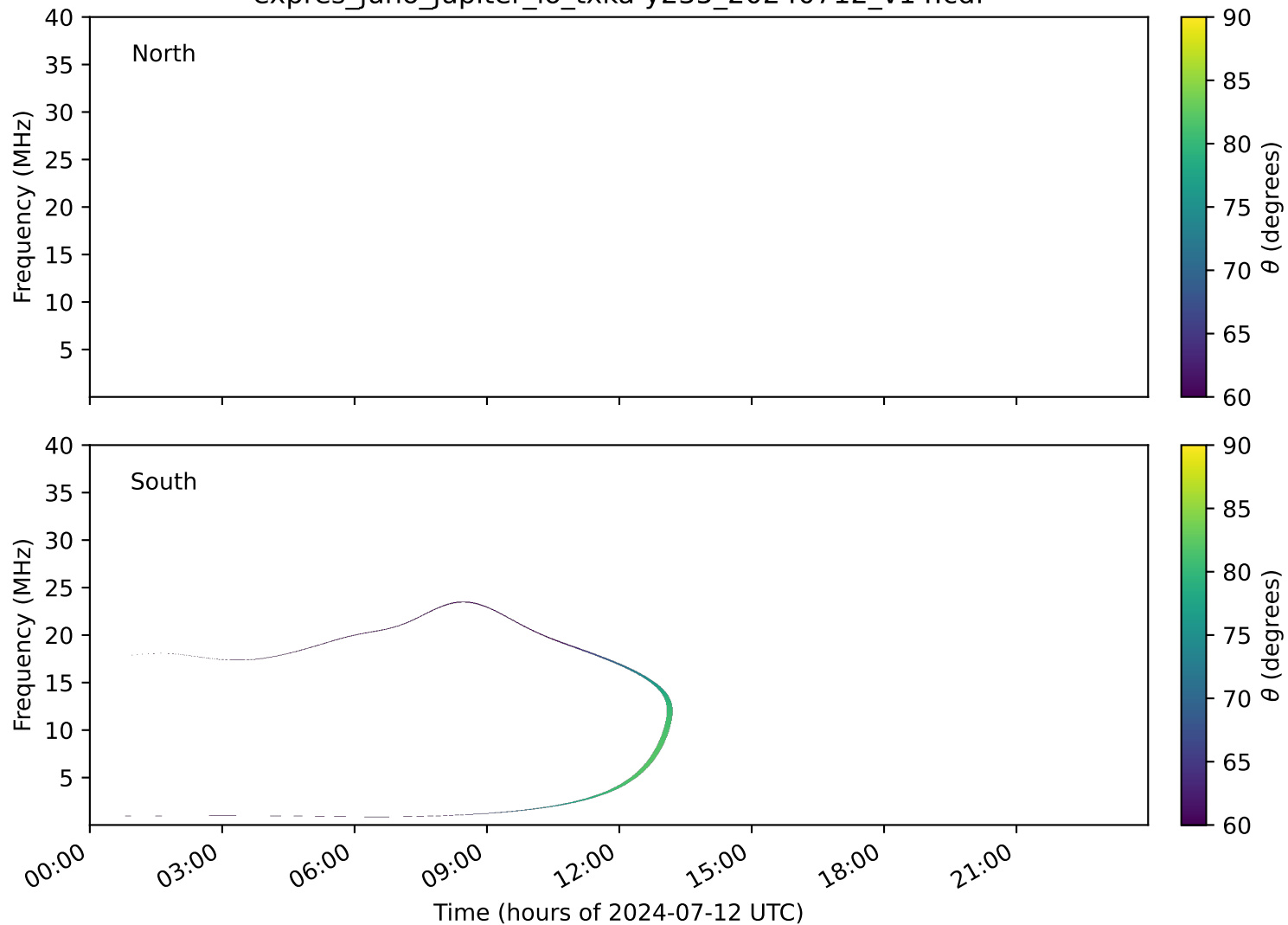
expres_juno_jupiter_io_txka-y235_20240712_v14.cdf
