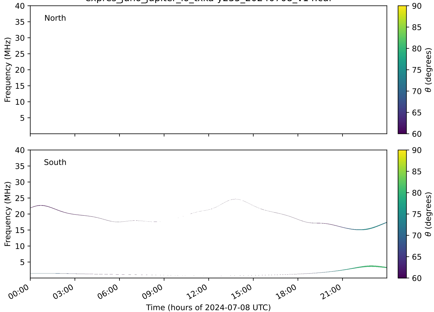
expres_juno_jupiter_io_txka-y235_20240708_v14.cdf
