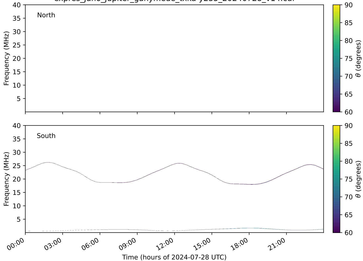
expres_juno_jupiter_ganymede_txka-y235_20240728_v14.cdf
