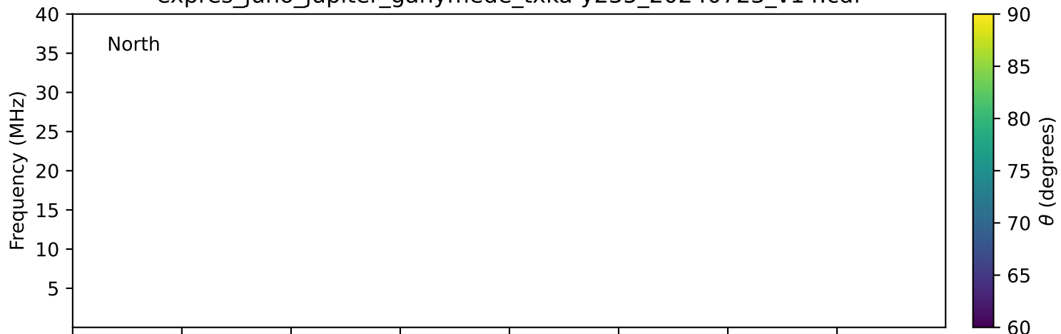
expres_juno_jupiter_ganymede_txka-y235_20240723_v14.cdf
