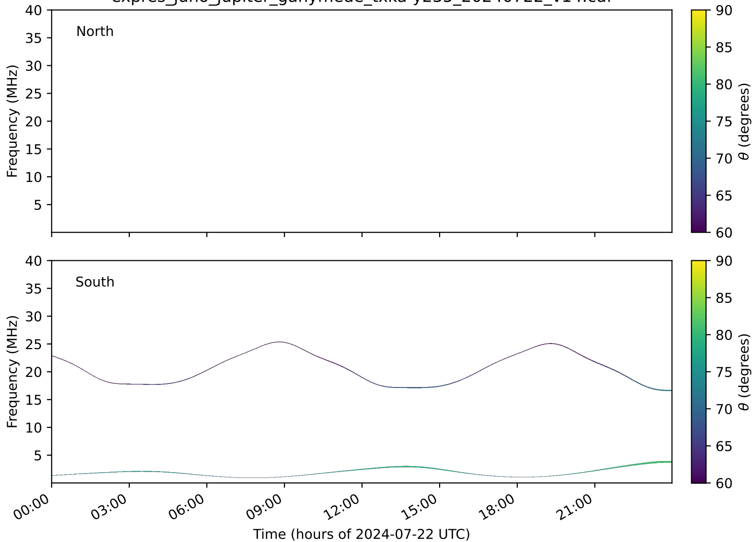
expres_juno_jupiter_ganymede_txka-y235_20240722_v14.cdf
