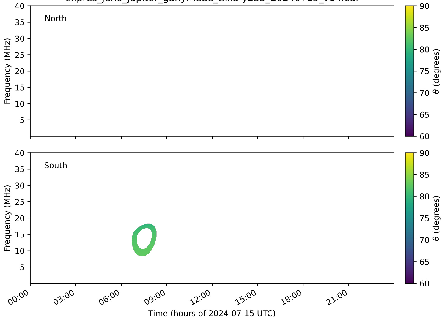
expres_juno_jupiter_ganymede_txka-y235_20240715_v14.cdf
