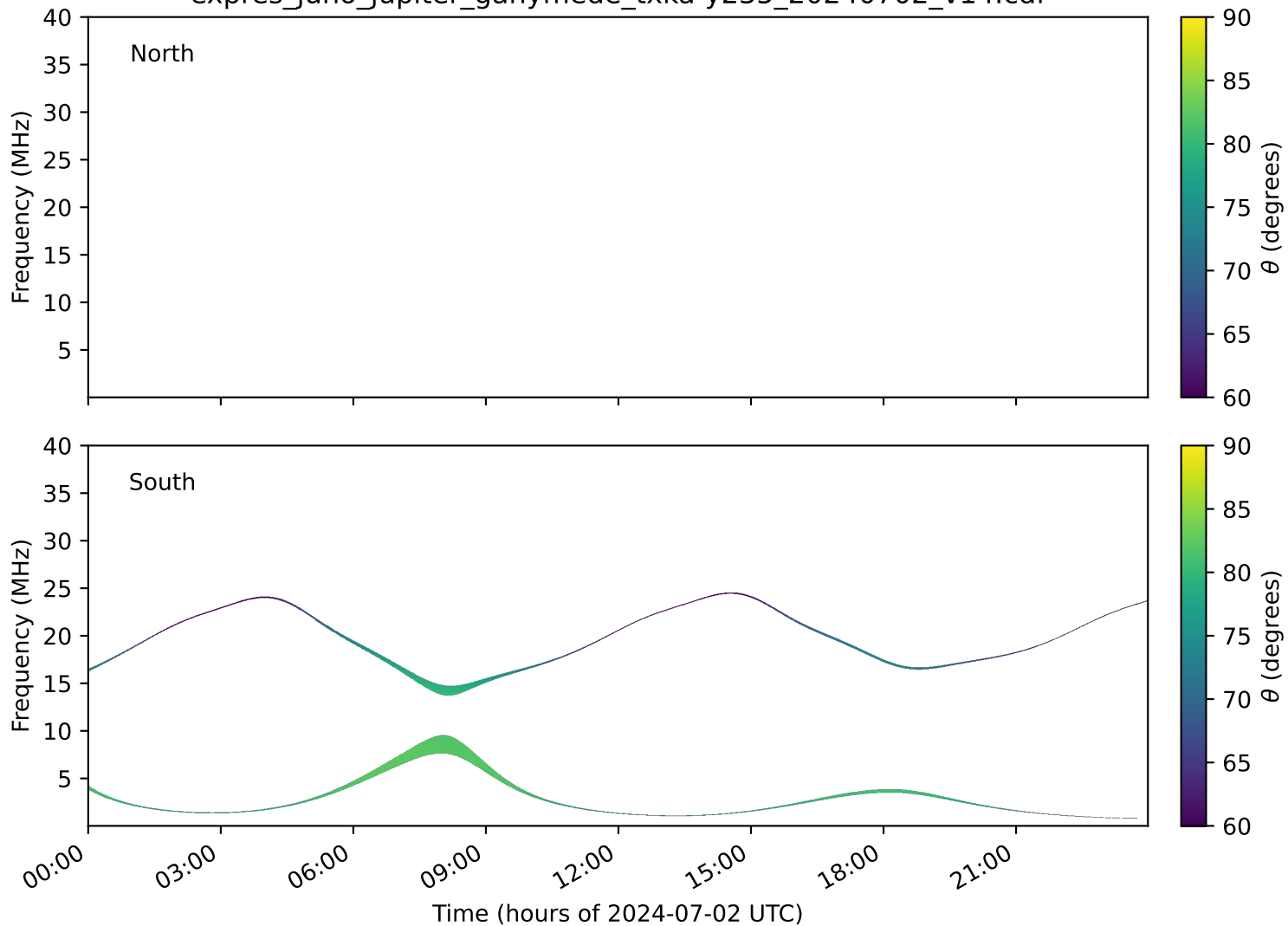
expres_juno_jupiter_ganymede_txka-y235_20240702_v14.cdf
