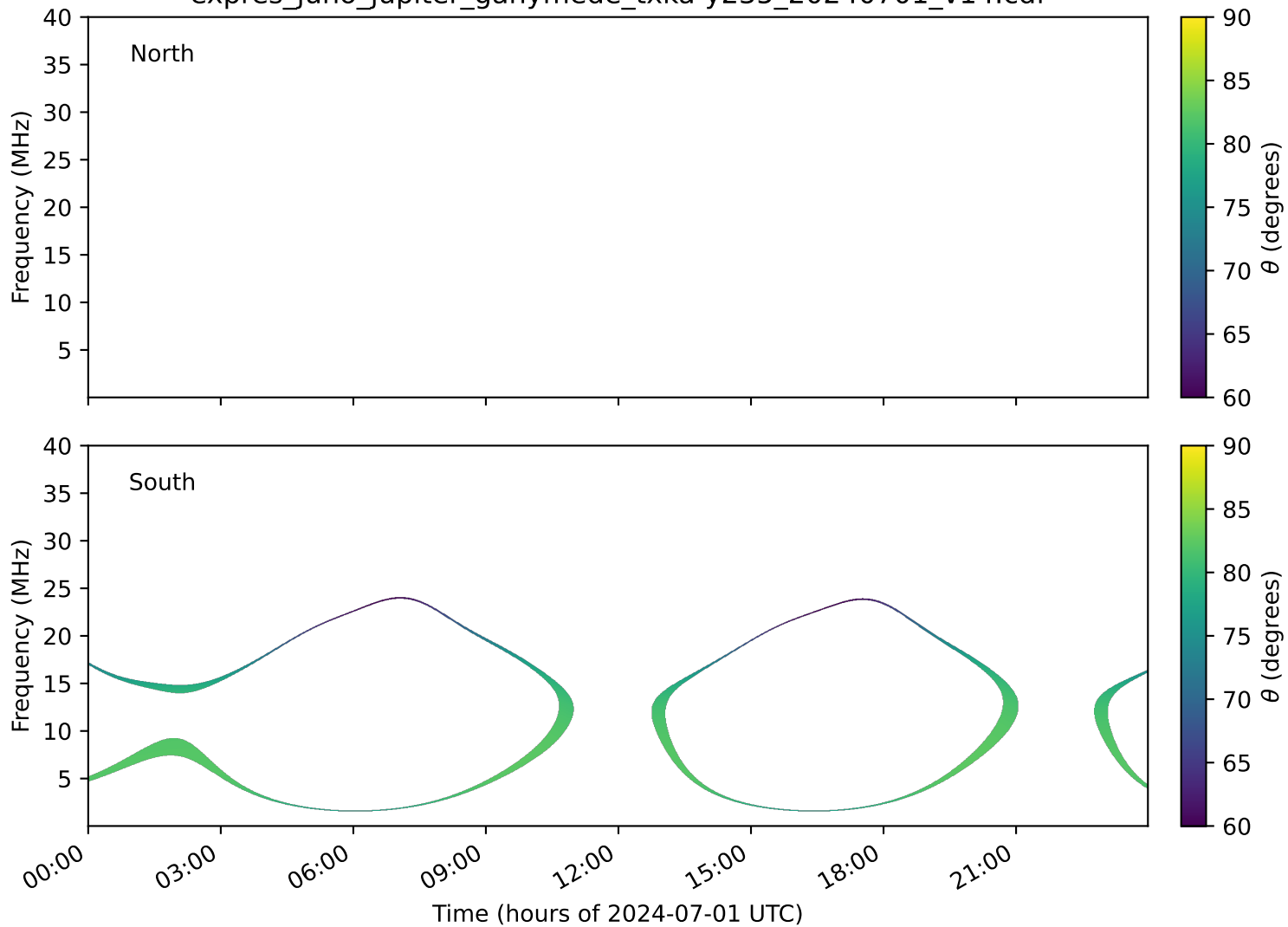
expres_juno_jupiter_ganymede_txka-y235_20240701_v14.cdf
