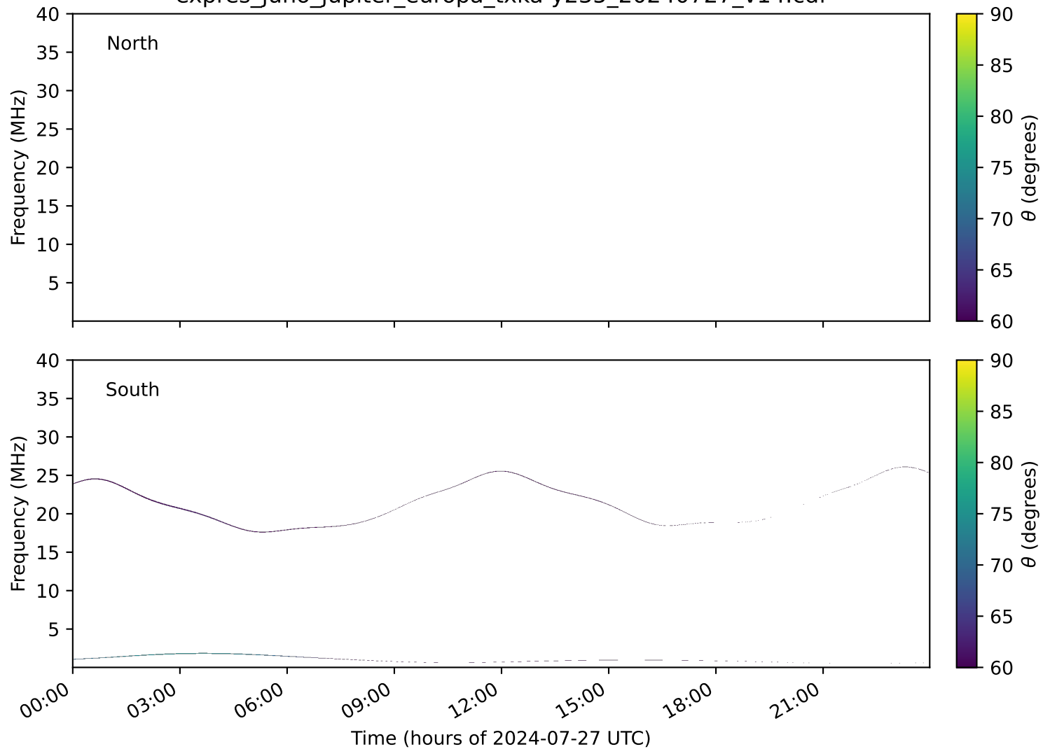
expres_juno_jupiter_europa_txka-y235_20240727_v14.cdf
