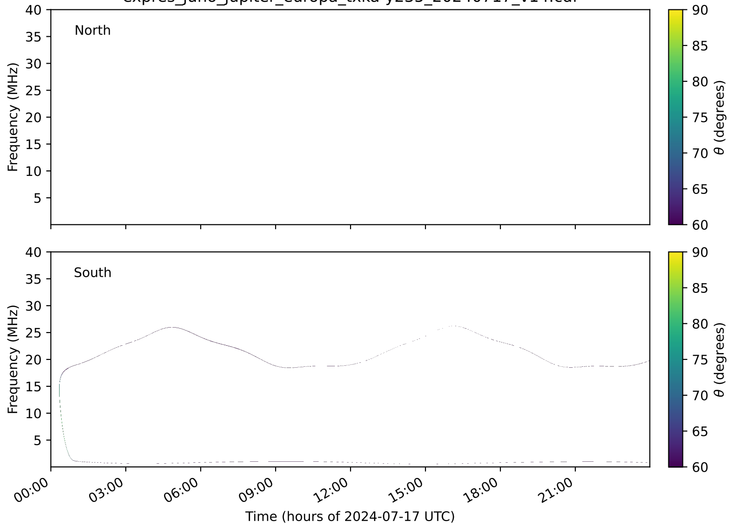
expres_juno_jupiter_europa_txka-y235_20240717_v14.cdf
