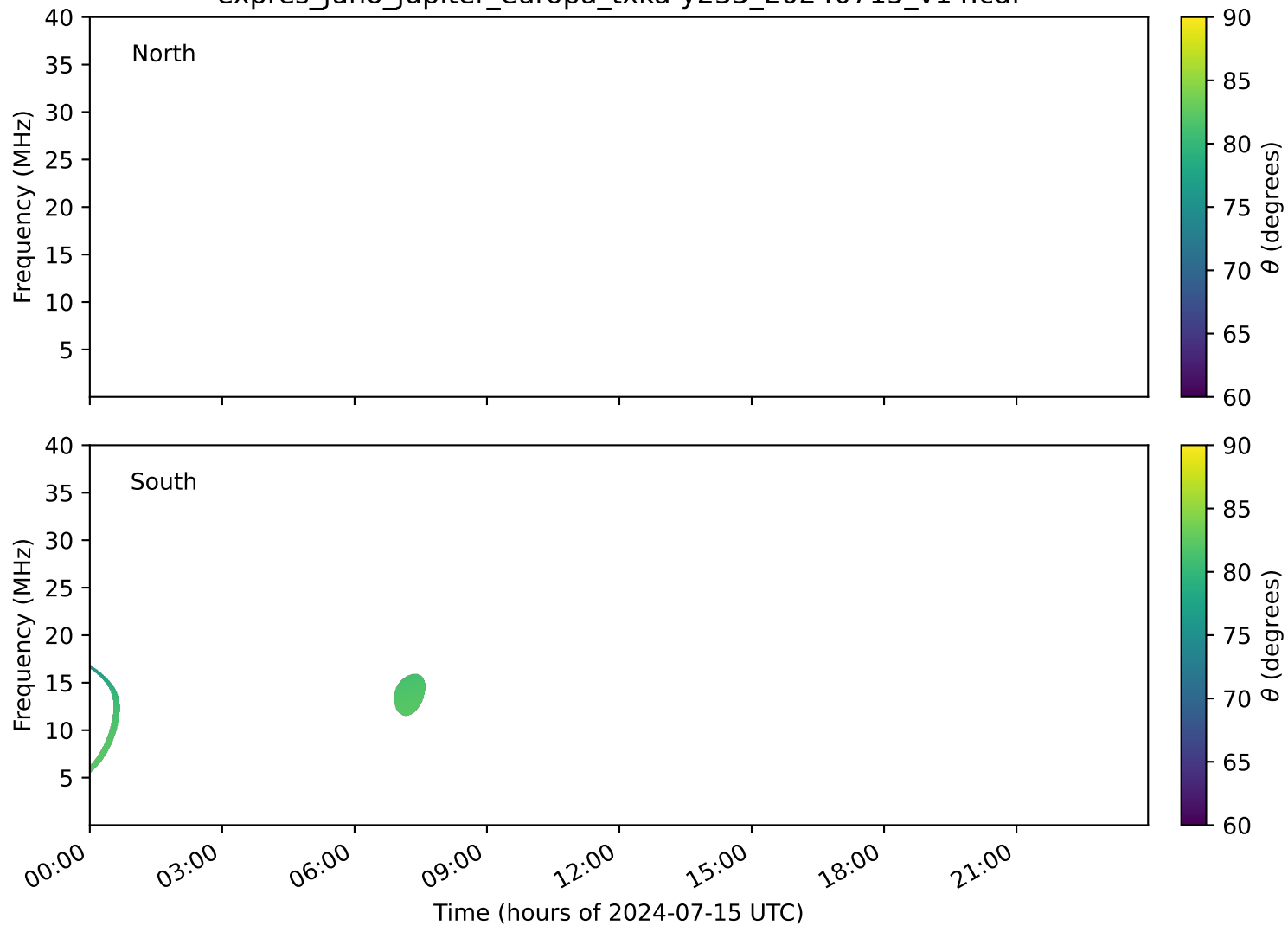
expres_juno_jupiter_europa_txka-y235_20240715_v14.cdf
