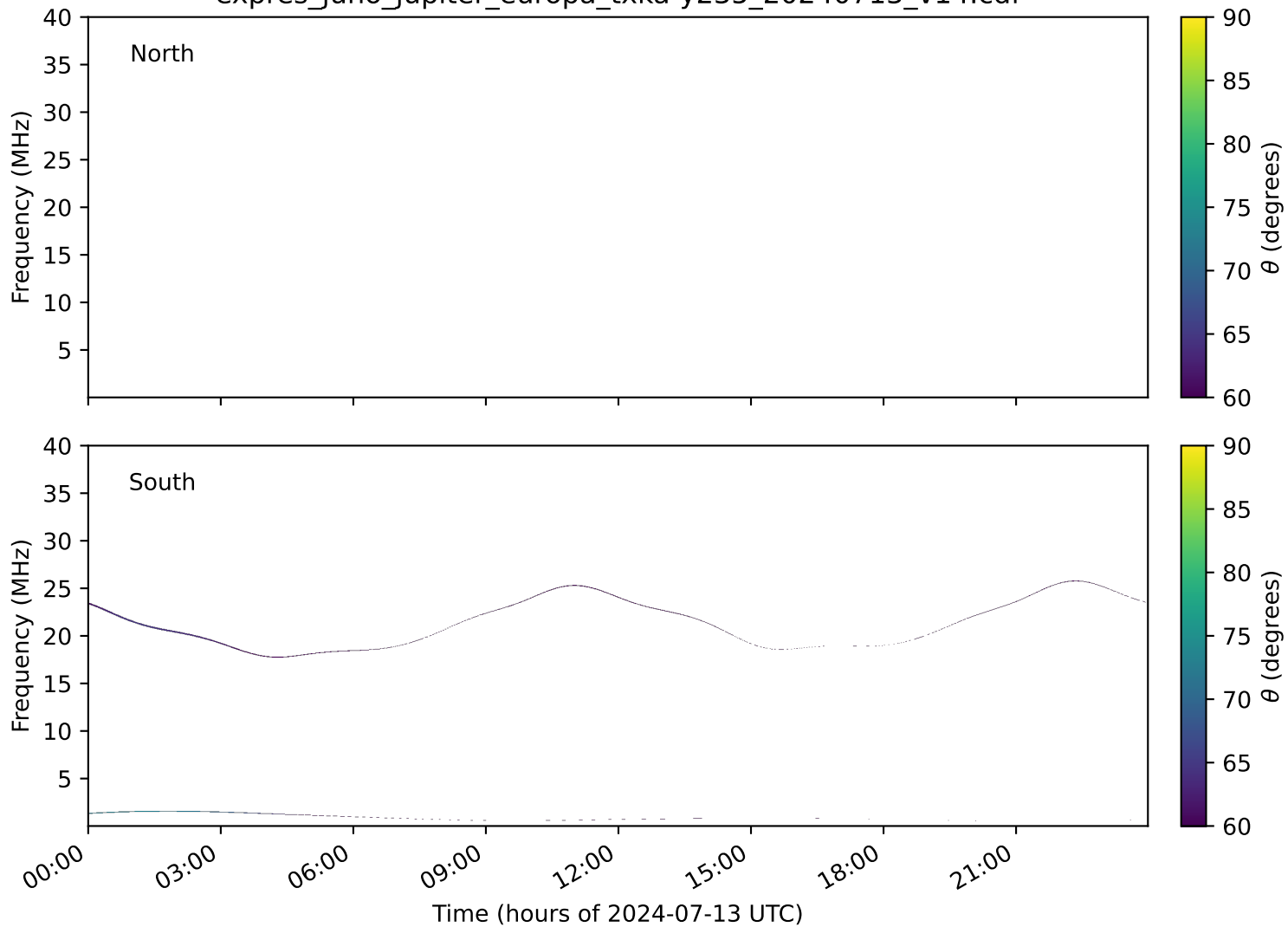
expres_juno_jupiter_europa_txka-y235_20240713_v14.cdf
