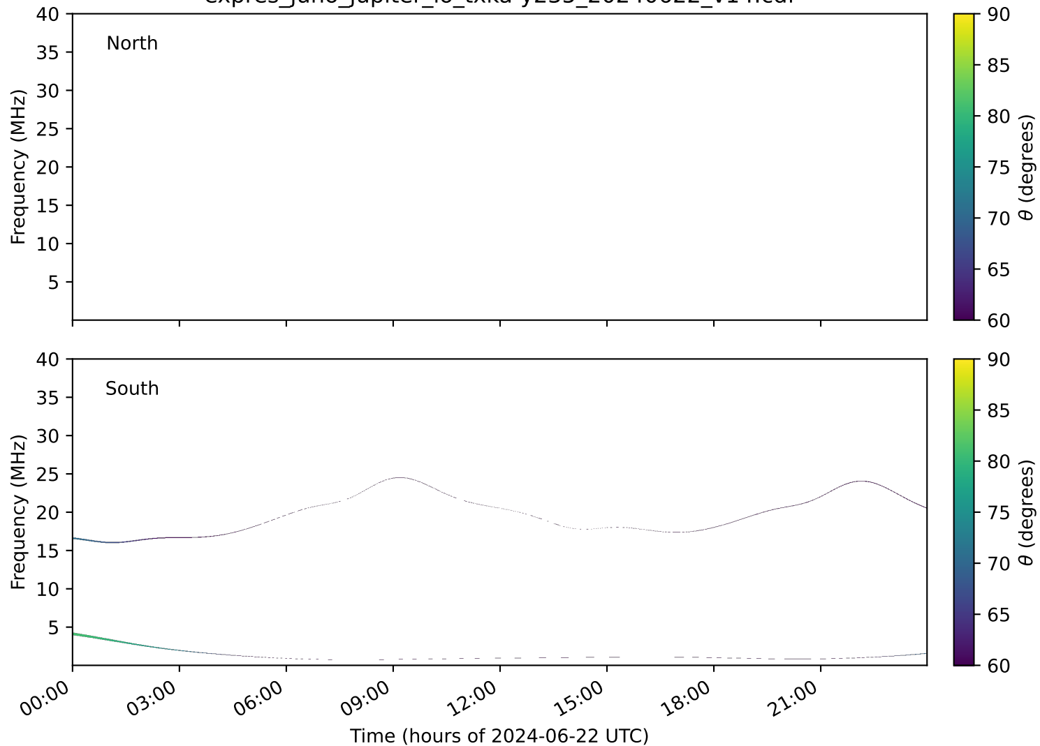
expres_juno_jupiter_io_txka-y235_20240622_v14.cdf
