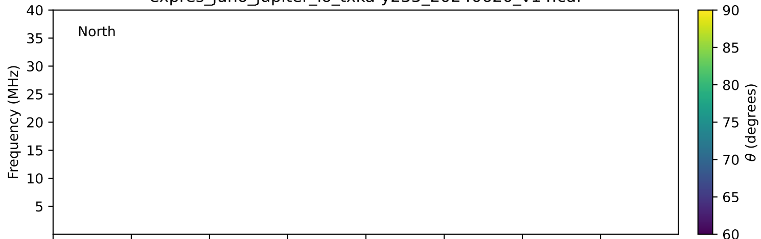
expres_juno_jupiter_io_txka-y235_20240620_v14.cdf
