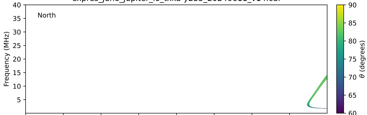
expres_juno_jupiter_io_txka-y235_20240611_v14.cdf
