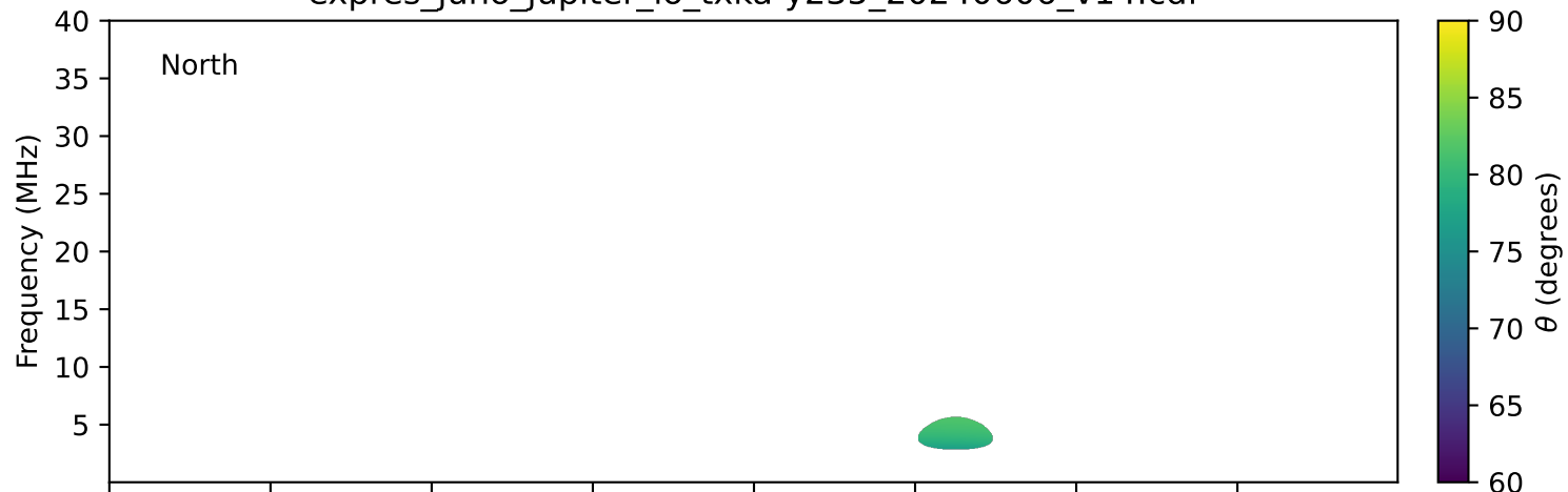
expres_juno_jupiter_io_txka-y235_20240606_v14.cdf
