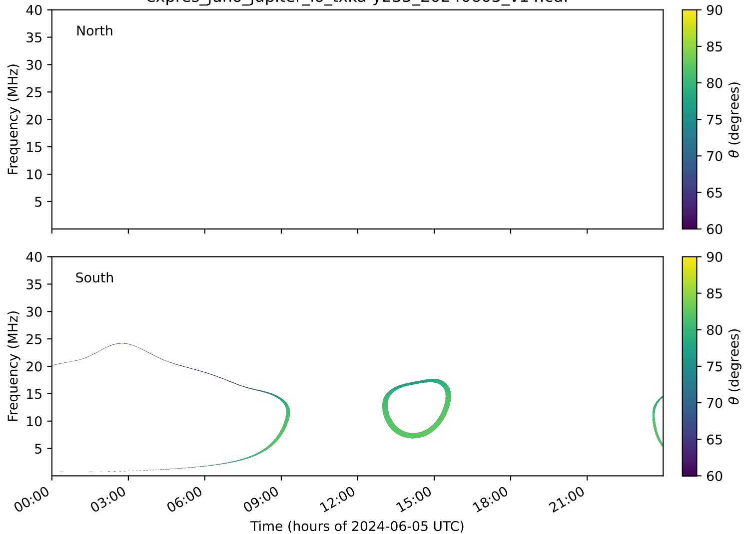
expres_juno_jupiter_io_txka-y235_20240605_v14.cdf
