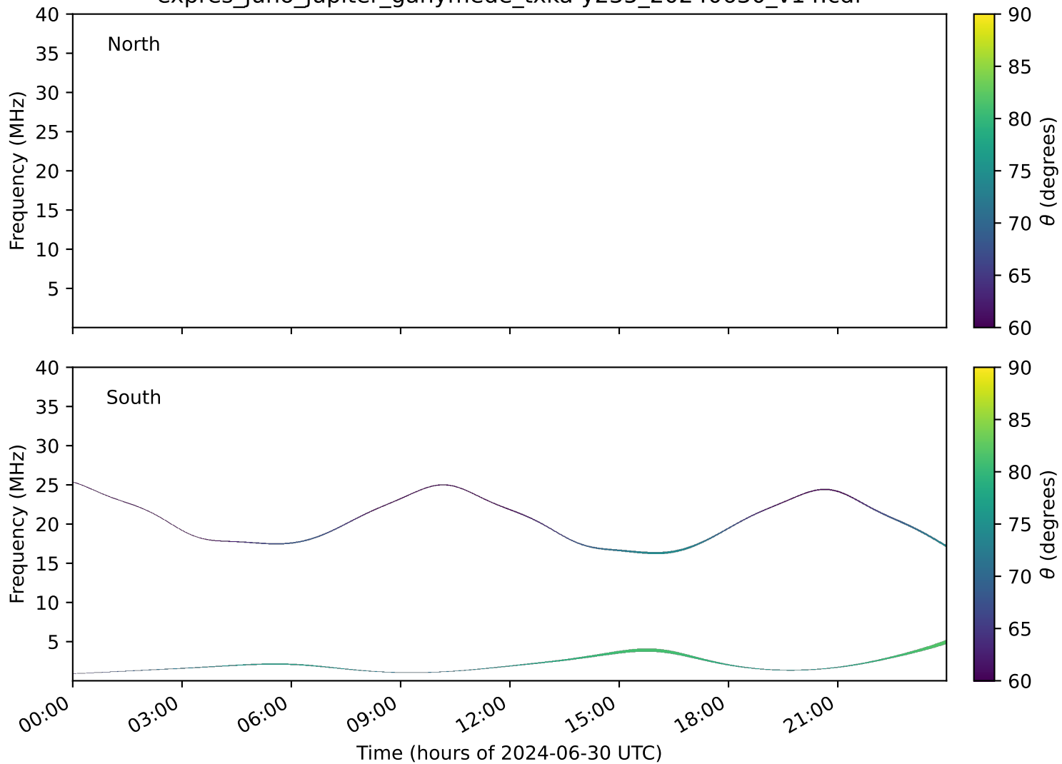
expres_juno_jupiter_ganymede_txka-y235_20240630_v14.cdf
