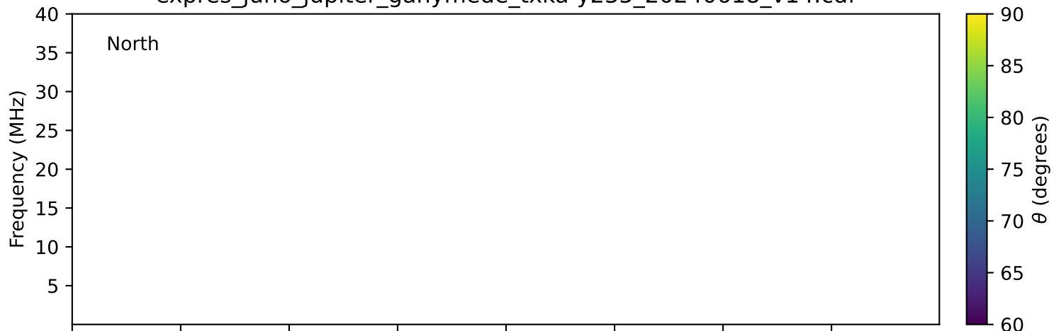
expres_juno_jupiter_ganymede_txka-y235_20240618_v14.cdf
