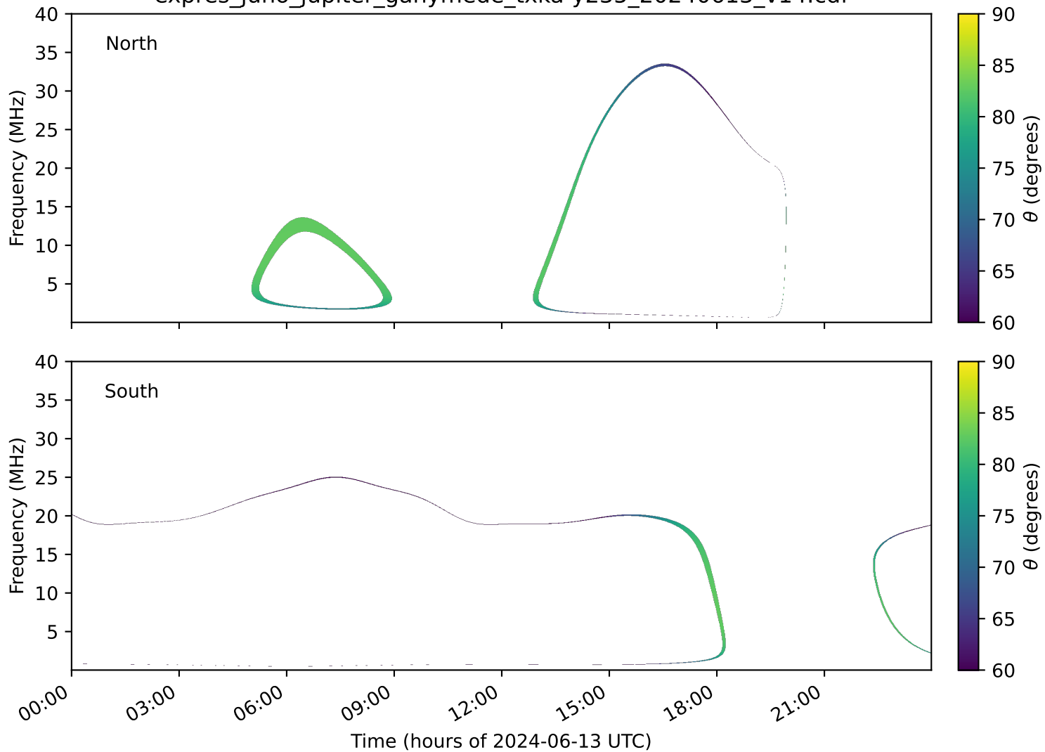
expres_juno_jupiter_ganymede_txka-y235_20240613_v14.cdf
