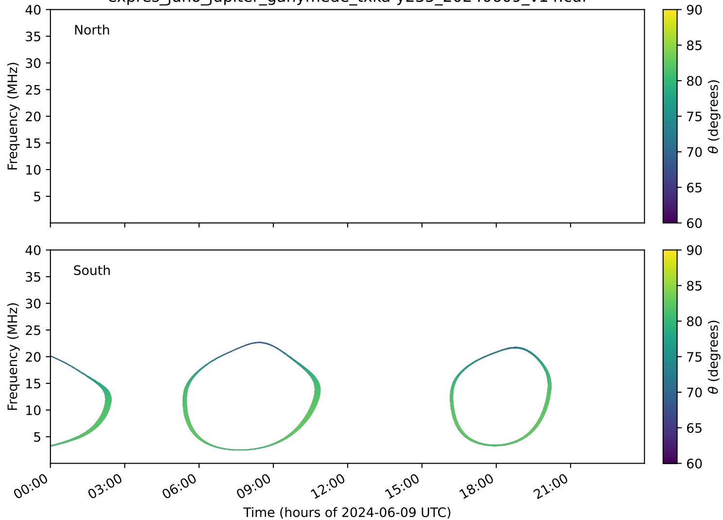
expres_juno_jupiter_ganymede_txka-y235_20240609_v14.cdf
