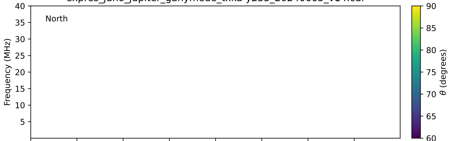
expres_juno_jupiter_ganymede_txka-y235_20240605_v14.cdf
