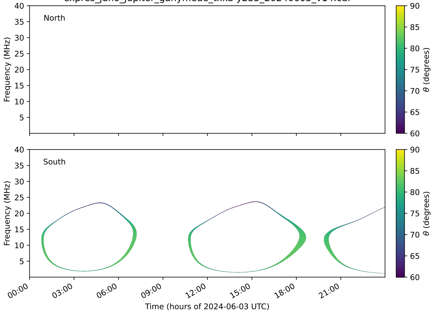
expres_juno_jupiter_ganymede_txka-y235_20240603_v14.cdf
