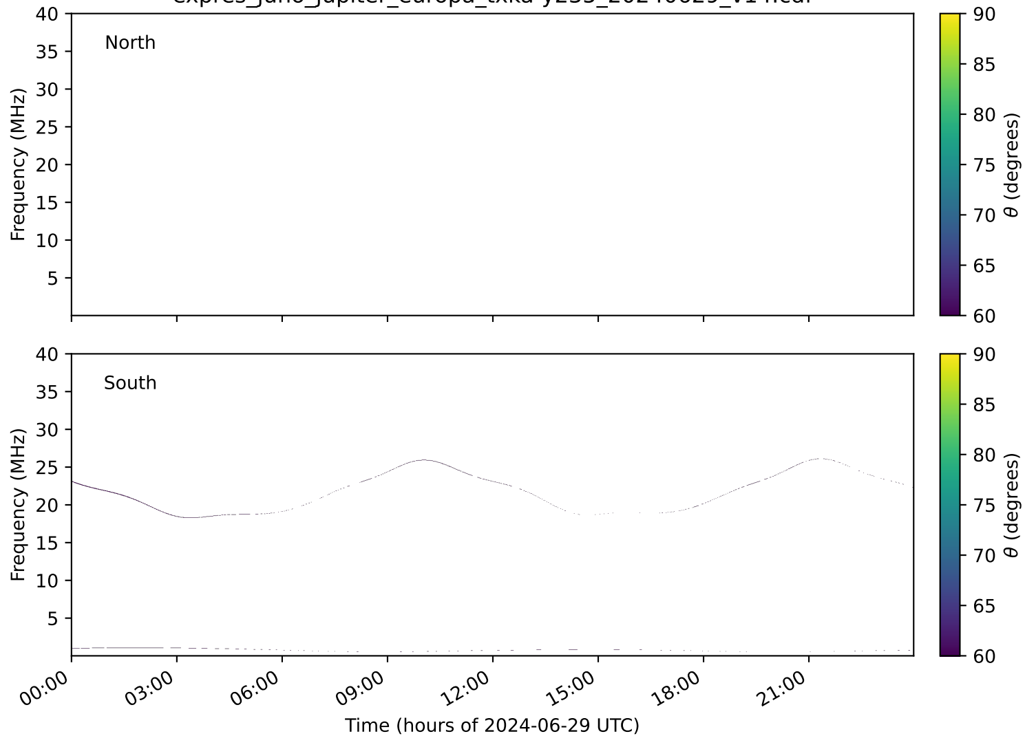
expres_juno_jupiter_europa_txka-y235_20240629_v14.cdf
