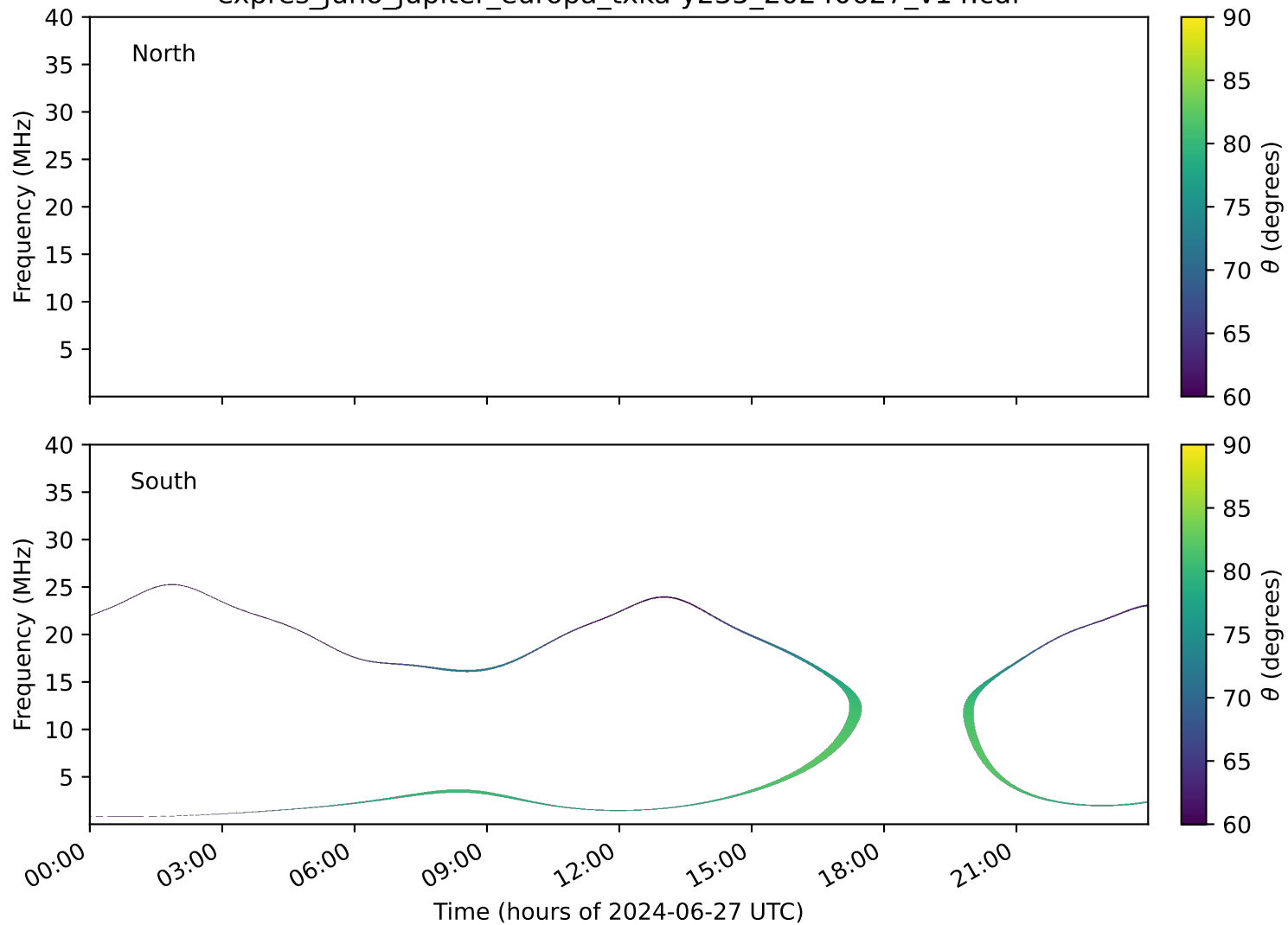
expres_juno_jupiter_europa_txka-y235_20240627_v14.cdf
