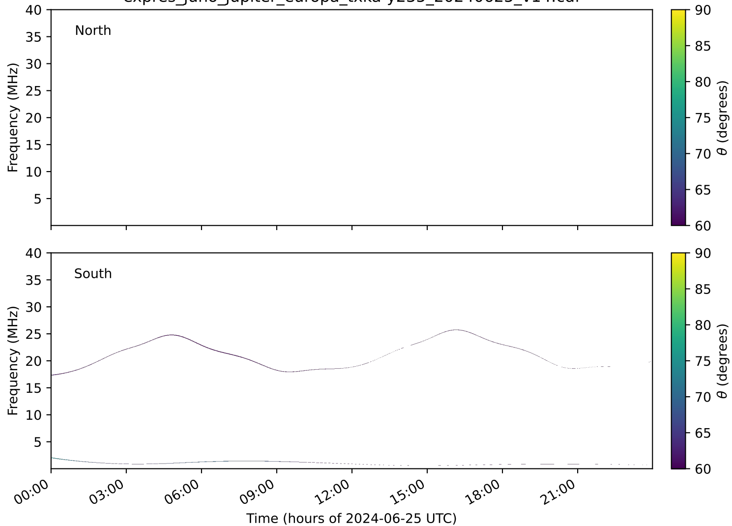
expres_juno_jupiter_europa_txka-y235_20240625_v14.cdf
