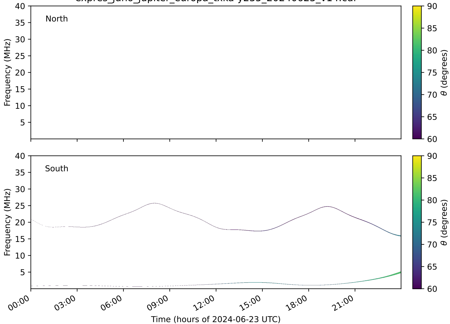
expres_juno_jupiter_europa_txka-y235_20240623_v14.cdf
