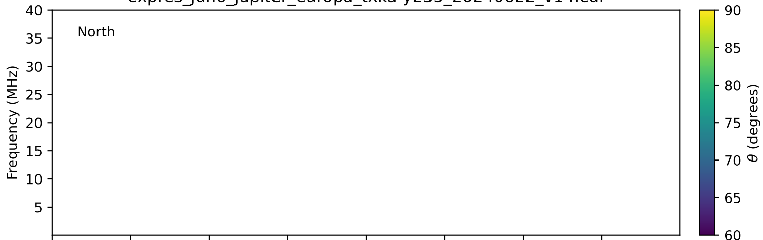
expres_juno_jupiter_europa_txka-y235_20240622_v14.cdf
