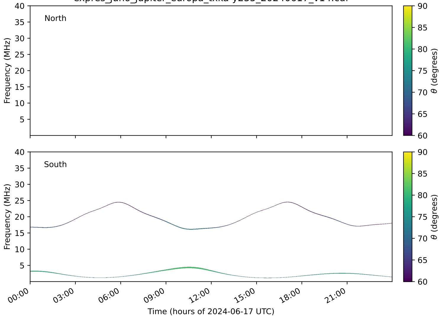
expres_juno_jupiter_europa_txka-y235_20240617_v14.cdf
