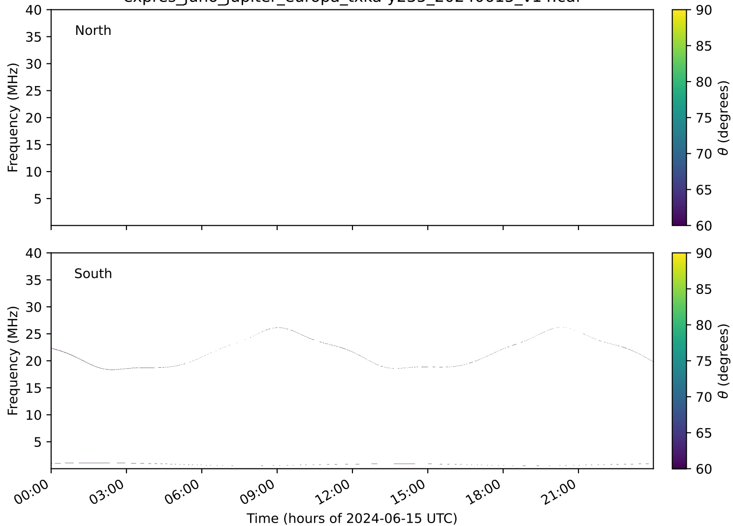
expres_juno_jupiter_europa_txka-y235_20240615_v14.cdf
